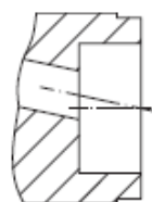
Fig. 6A1...3 with socket weld ends
