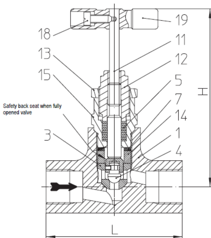
Fig. 6A1...2 with screwed sockets
