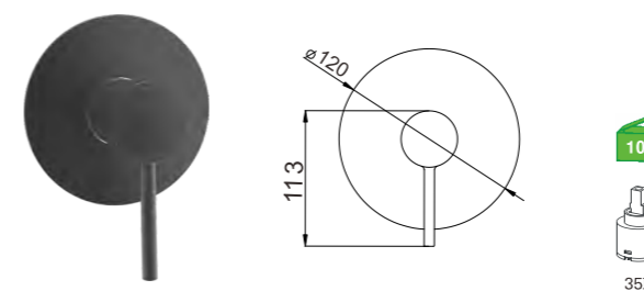
D26FK13BL(B) Monocomando embutido 1 via Built-in mixer Monomando empotrado 1 via
