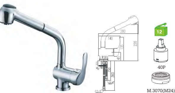
C17DF7C Monocomando lava-loiça com chuveiro Kitchen mixer with pull out shower Monomando fregadero extraíble
