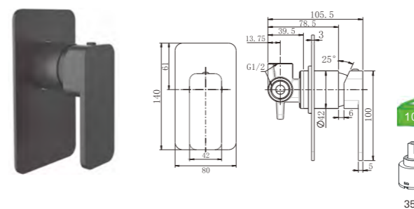
D21RP13BL(B) Monocomando embutido 1 via Built-in mixer Monomando empotrado 1 via
