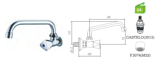
H110339C Torneira à parede bica alta 1 água Wall mounted faucet Grifo pared 1 agua BICA ---3069
