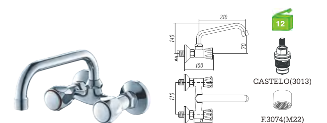
H110299C Misturadora lava-loiça à parede bica alta – 11cm Wall mounted kitchen mixer (11cm) Monobloc fregadero pared (caño alto) – 11cm BICA ---3069
