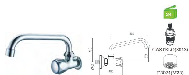
H110229C Torneira à parede bica alta 1 água Wall mounted faucet Grifo pared 1 agua BICA ---3069
