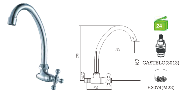
H11T19C Torneira à parede bica alta 1 água Wall mounted faucet Grifo pared 1 agua BICA ---3062
