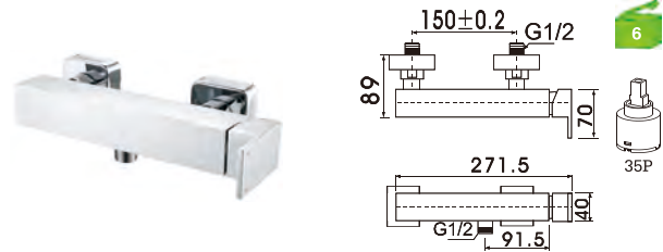
C53FX3C Monocomando duche
