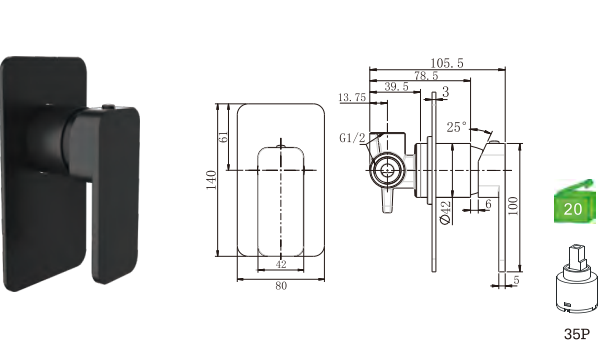
D21RP13BL(B) Monocomando embutido 1 via Built-in mixer Monomando empotrado 1 via
