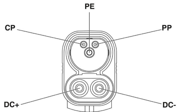
1-2 CCS 2 Charging Connector
