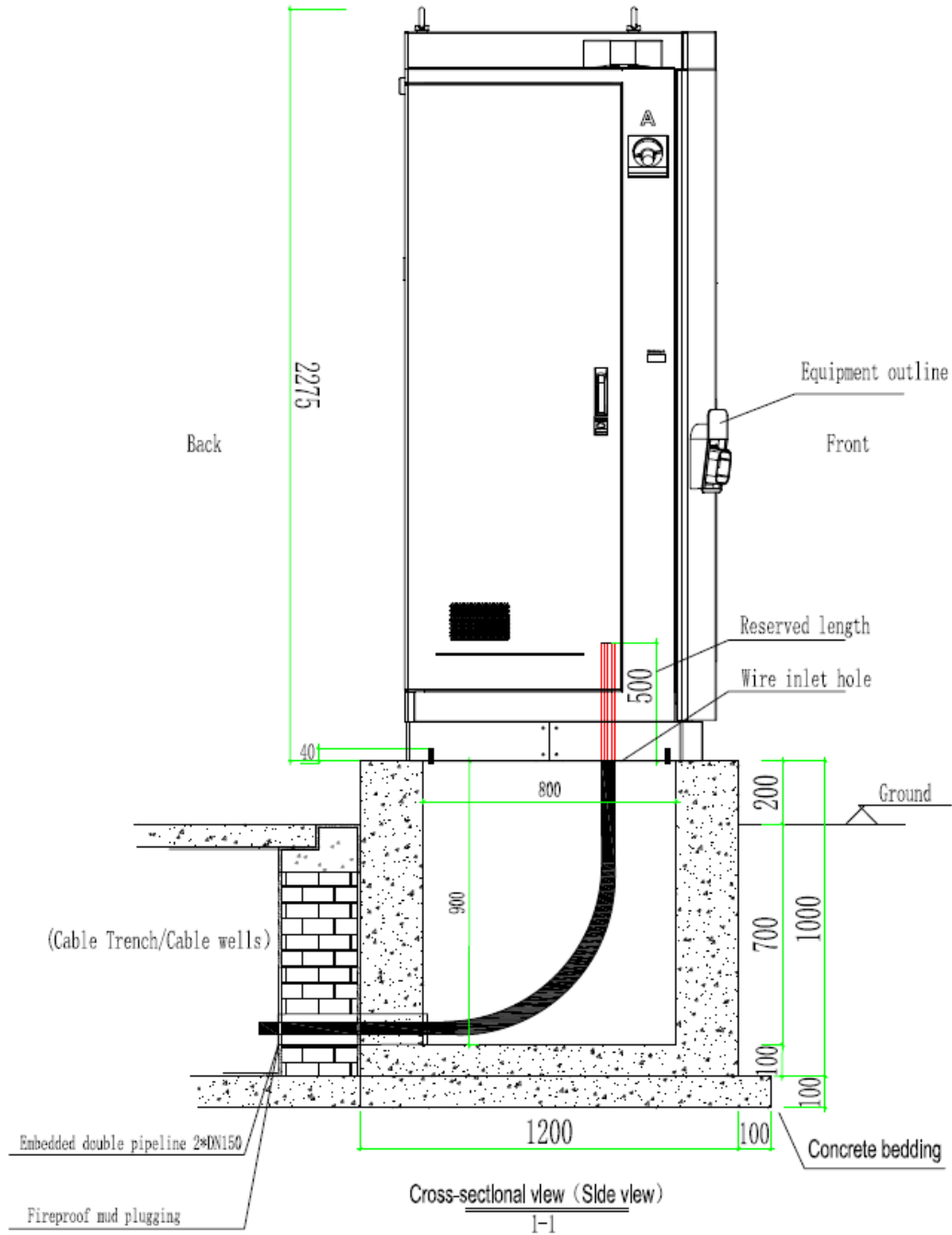
2-1 Concrete Foundation Profile Map
