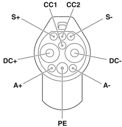
1-5 GB/T Charging Connector
