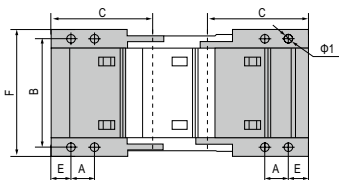
F-F 型接头 F-F type bracket
