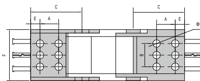
X 8 型接头 X 8 type bracket
