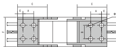
X 6-1 型接头 X 6-1 type bracket
