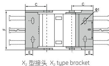
X 2 型接头 X 2 type bracket
