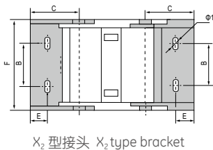
X 2 型接头 X 2 type bracket
