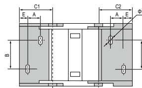
X 6 型接头 X 6 type bracket
