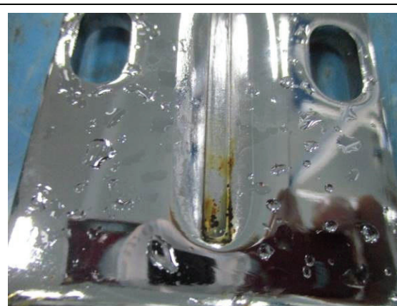
Sample #1 after salt spray tests - View 6
