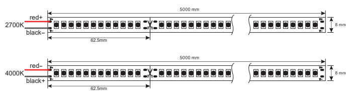
Circuit Diagram
