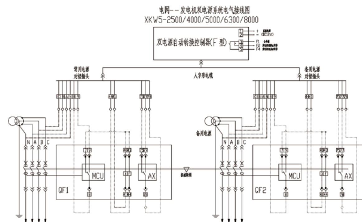
XKW5-2000 及以上断路器 XKW5-2000 and above circuit breaker
