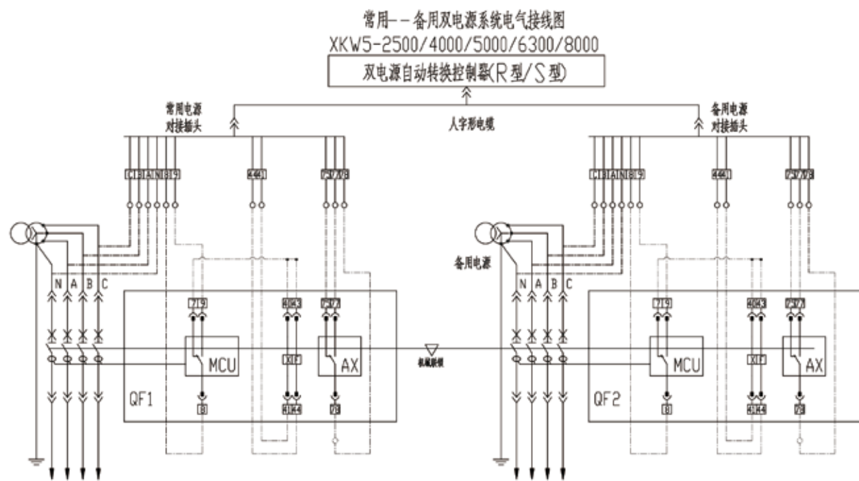
XKW5-2000 及以上断路器 XKW5-2000 and above circuit breaker
