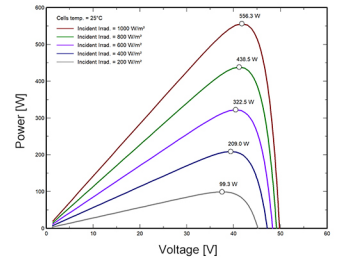
P-V CURVE (555W)
